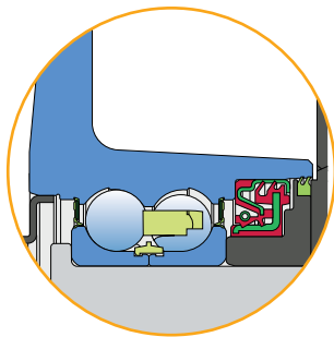
Sheet metal shield + RS seal / RS seal + Dirtblock seal + Double lip seal + Forged cover plate
