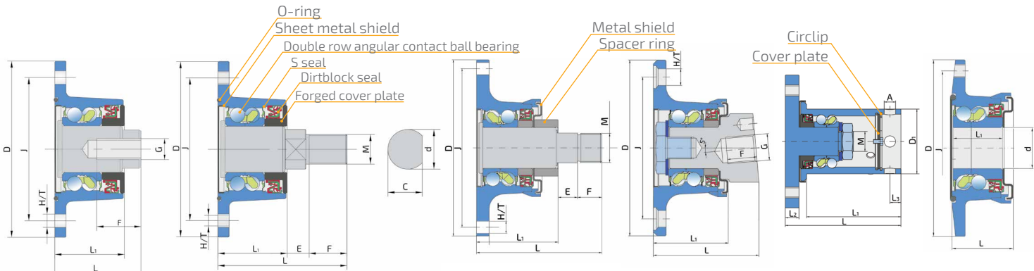
Figure 1 C= 75.86 kN *C= 66.35 kN Co=66.2 kN Co=56.49 kN Figure 2 C= 75.86 kN Co=66.2 kN Figure 3 C= 75.86 kN Co=66.2 kN Figure 4 C= 75.86 kN Co=66.2 kN Figure 5 C= 75.86 kN Co=66.2 kN Figure 6 C= 66.35 kN Co=56.49 kN
