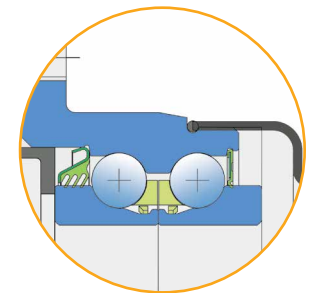
Plastic cover + 3-lip seal/RS seal + Threaded metal cap
