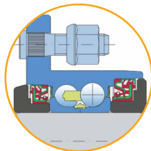
Forged cover plate + Dirtblock seal + RS seal/ RS seal + Dirtblock seal + Forged cover plate
